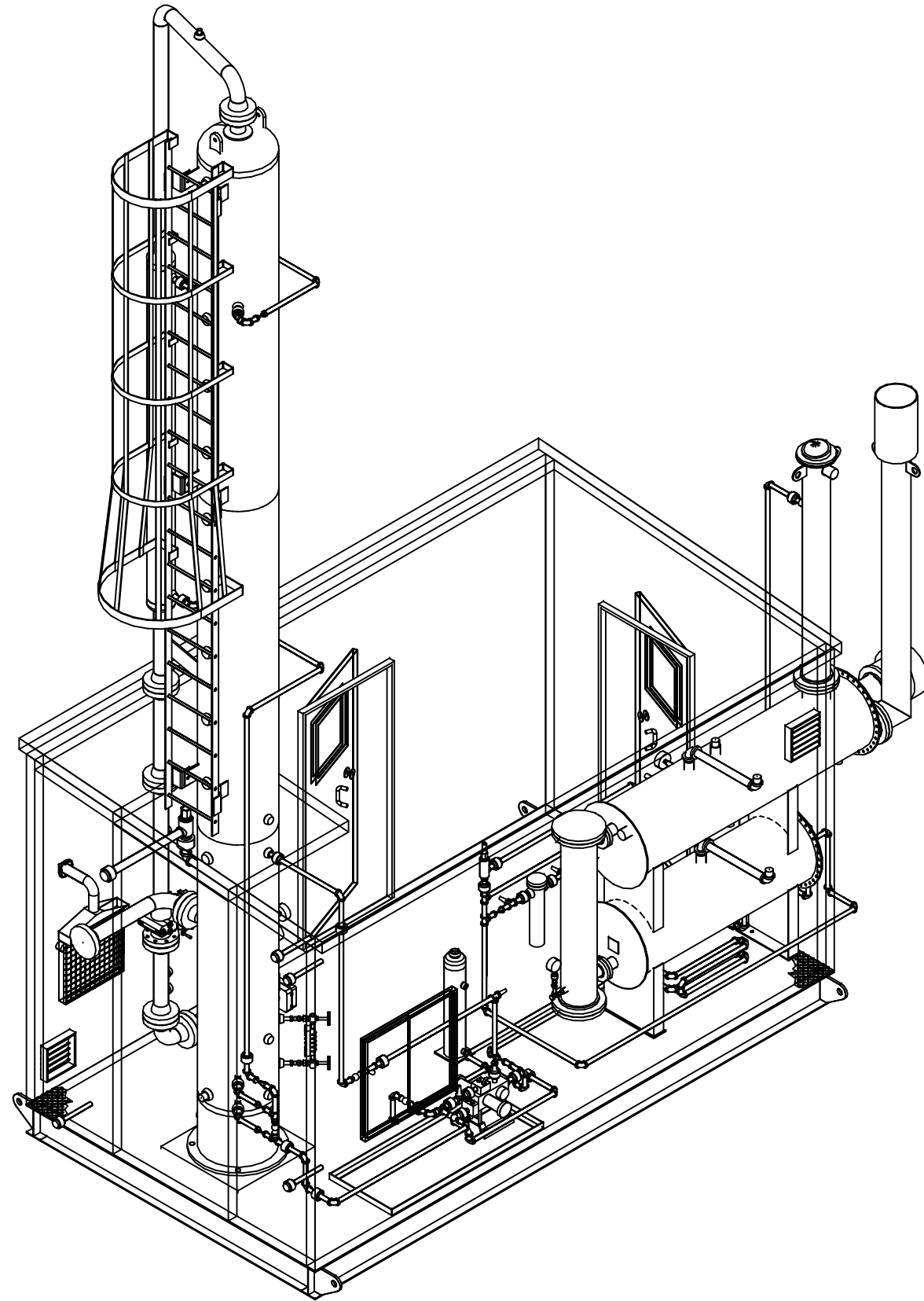
SW ISOMETRIC VIEW
