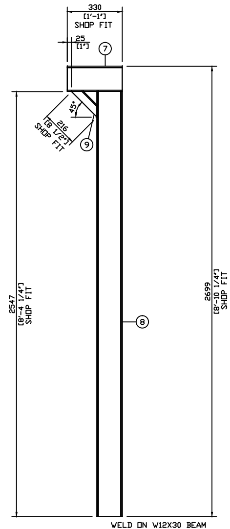
PS-06 DETAIL SCALE 1:10
