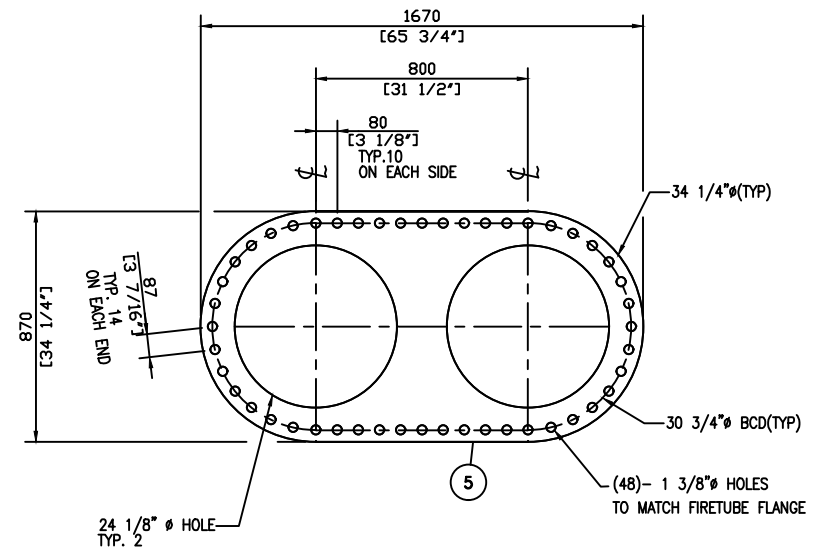
FIRETUBE COVER DETAIL
