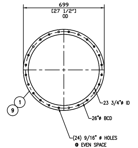
BURNER FLANGE & GASKET
