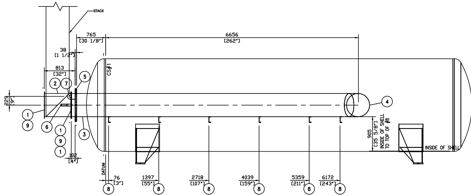
FIRETUBE ASSY. ELEVATION VIEW
